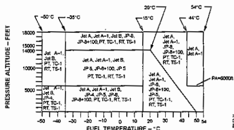
Fig. 2-3 Temperature limits for approved primary fuels
