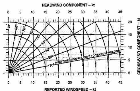
Fig. 1-7 Wind Component Chart
