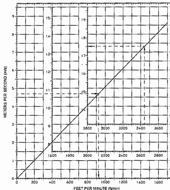
Fig. 1-3 Conversion chart: meters/second (m/s) – feet/minute (ft/min)
