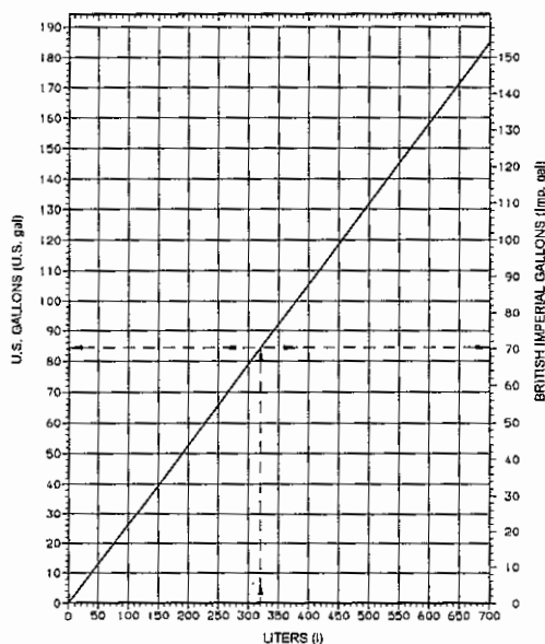
Fig. 1-5 Conversion chart: liters (l) – U.S. gallons (U.S. gal) – imp. gallons (imp. gal)
