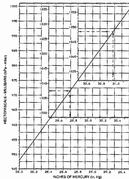
Fig. 1-6 Conversion chart: Hectopascals (hPa) – inches of Mercury (in. Hg)
