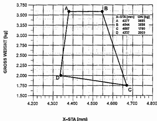
Fig. 2-1 Allowable CG envelope (longitudinal)
