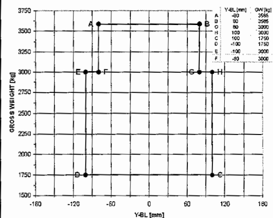
Fig. 2-2 Allowable CG envelope (lateral)
