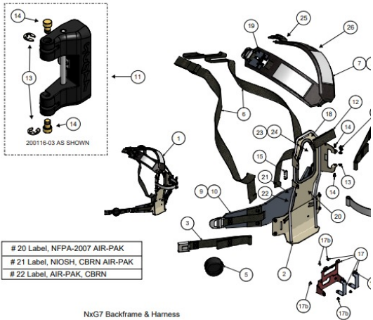
NxG7 Backframe & Harness P/N 200466-01 (Standard Harness) -02 (Spring Clips) Return to Table of Contents
